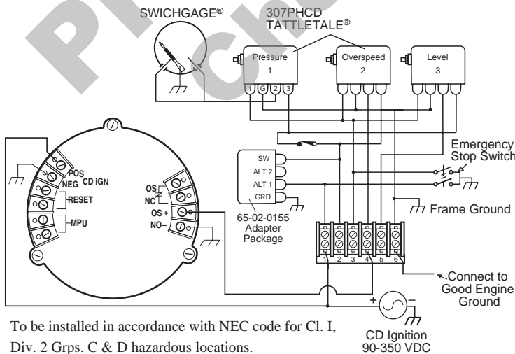
Figure 11: SHD45 with Normally Open S.C.R. output typical wiring for negative ground ignition systems.
